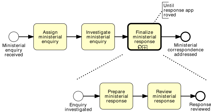
Fig. 4.5 The process model for addressing ministerial correspondence of Fig. 3.13 simplified using a loop activity
