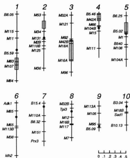
FIGURE 5.—Diagram of the ten teosinte-maize chromosomes showing the distribution of MMLs in this study. Distances between the MMLs are shown as r , the recombination fraction (see scale). Stippled blocks highlight regions with major effects on the morphological differences between maize and teosinte inflorescence architecture (see Figure 7). Prefixes indicate source of cloned MMLs as either University of Missouri-Columbia (M = UMC) or Brookhaven National Laboratory (B = BNL). Five isozyme loci ( Adk1 , Idh2 , Prx3 , Sad1 and Tpi3 ) are shown. Solid circles indicate the approximate positions of the centromeres (COE, HOISINGTON and NEUFFER 1990).
