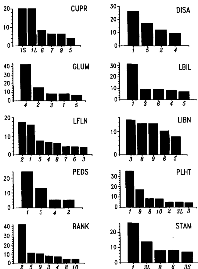
FIGURE 6.—Column graphs showing the number and magnitudes of significant associations between MTLs and the morphological traits. The heights of the columns represent the R^2 values from the regression analysis expressed as a percentage. The numbers below each column are the chromosome or chromosome arm on which the effect was seen. A key to the acronyms for the traits can be found in Table 1.
