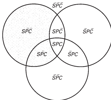
Figure 19-19 All seals are pessimists.
