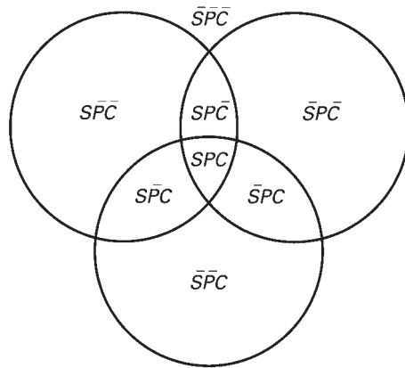
Figure 19-18 All the areas are identified.
