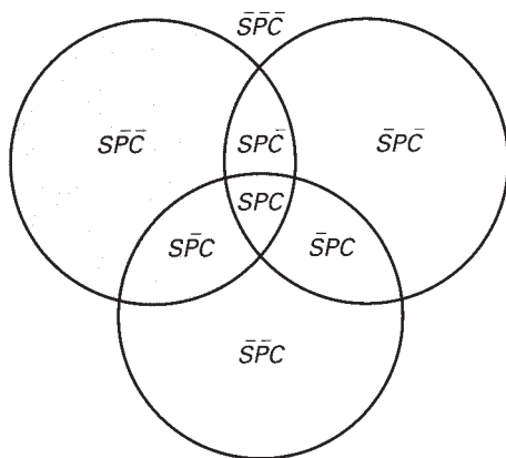
Figure 19-21 All seals are pessimists.
