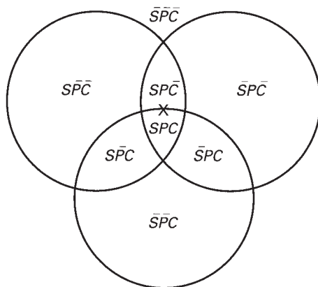
Figure 19-25 Some seals are pessimists.
