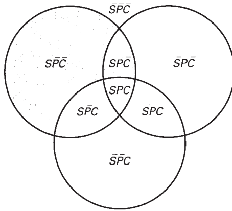
Figure 19-23 All seals are cribbage-cheaters.
