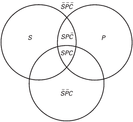
Figure 19-17 \bar{S}\bar{P}C , cribbage-cheaters who are non-seal and non-pessimist.
