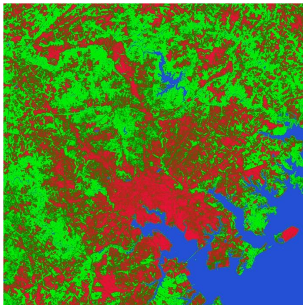
Figure 2B. Classified Landsat TM Image of Baltimore, Maryland, USA (Green-vegetation, Blue-Water Bodies, and Red-Urban)
